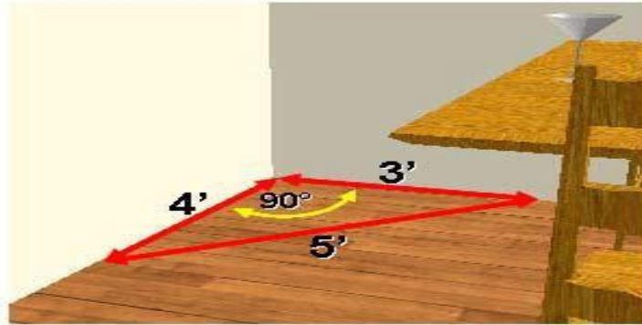
3-4-5 right angle
